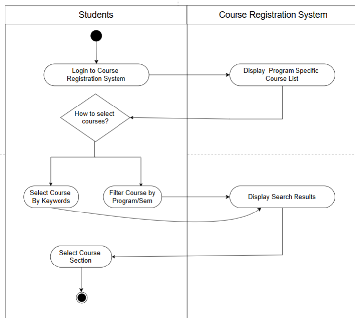
Figure 4.7.3 Activity Diagram for Course Registration & Application Portal
