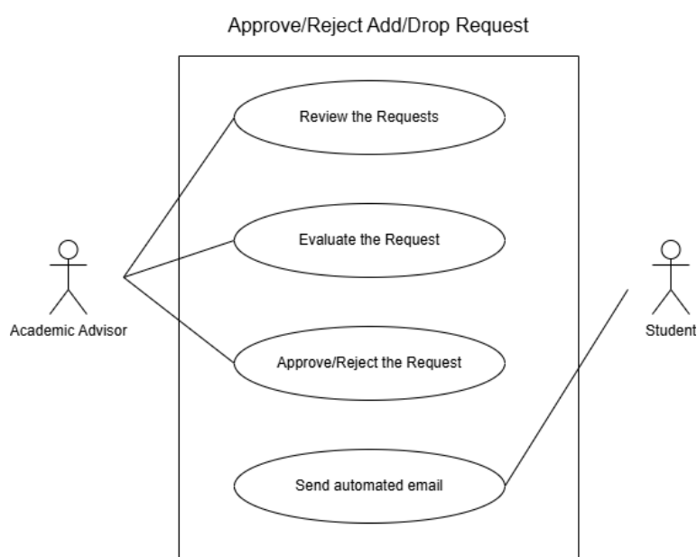
Figure 4.10.1 Use Case Diagram for Sub-Module Add/Drop Approval Workflow
