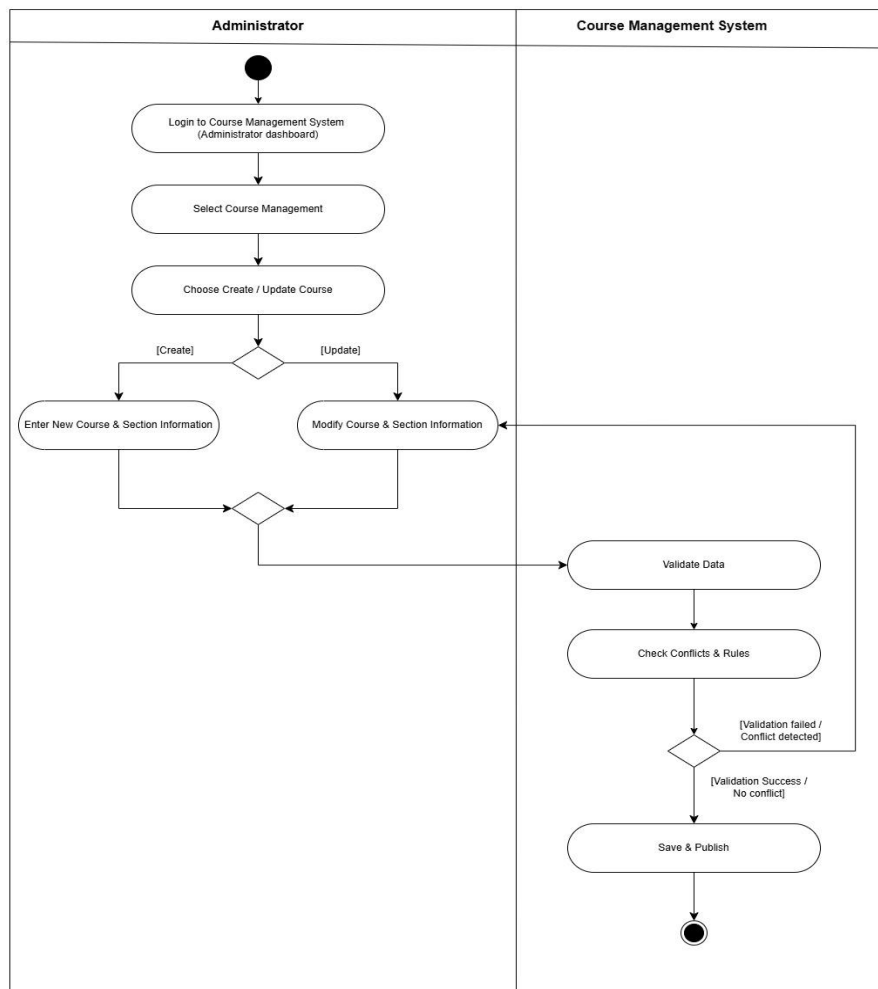
Figure 4.11.2 Activity Diagram for Sub-Module Course Master Data Administrator
