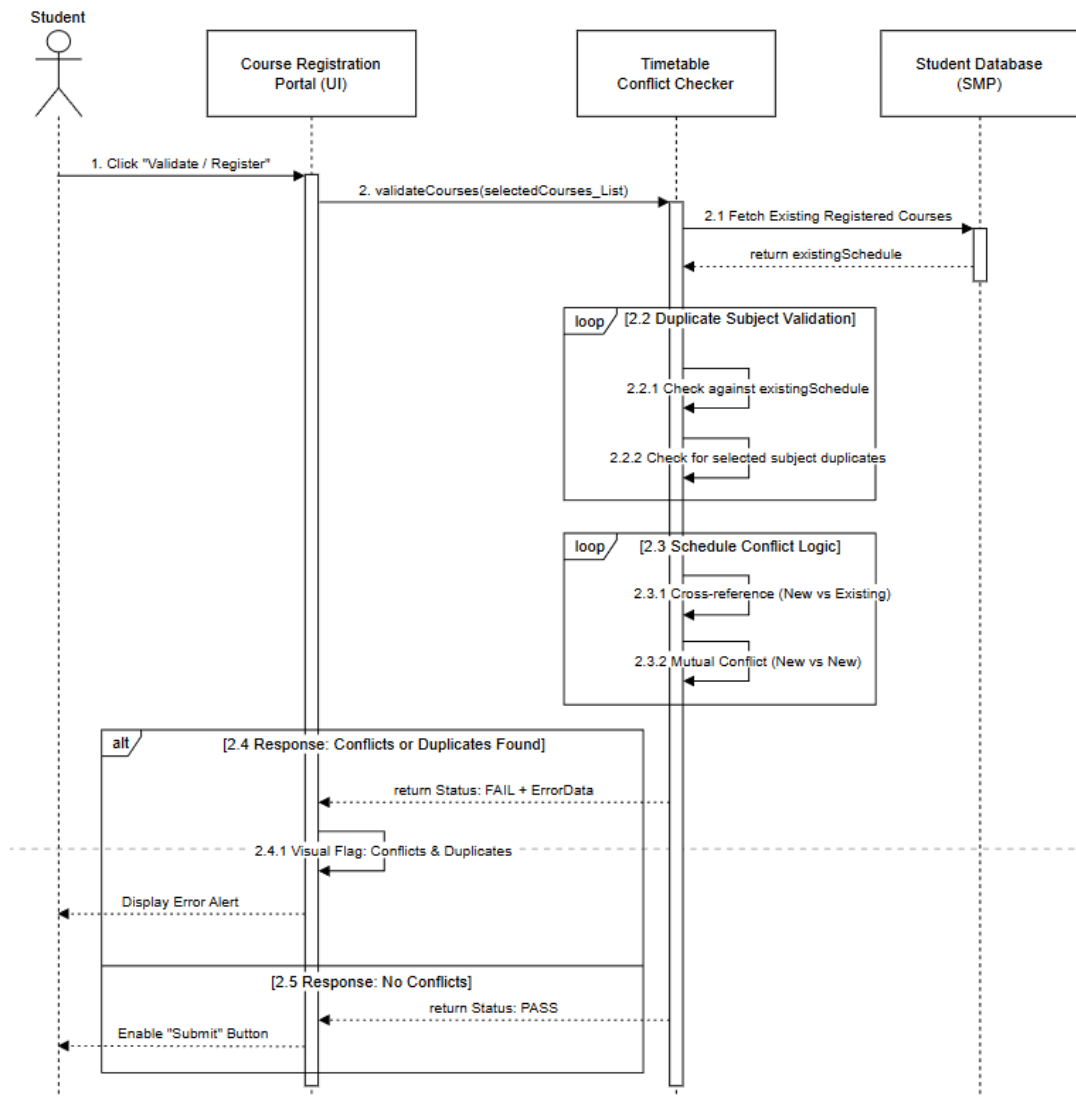
Figure 4.8.2 Sequence Diagram for Timetable Conflict Checker Module
