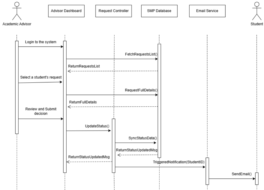
Figure 4.10.3 Sequence Diagram for Add/Drop Approval Workflow
