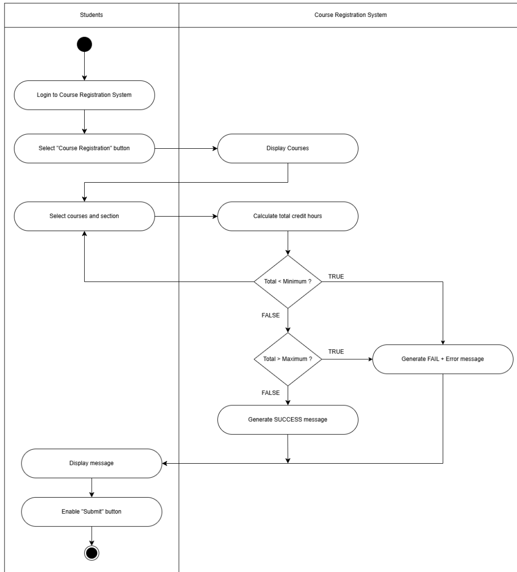
Figure 4.9.2 Activity diagram for Credit Hours Validator Module
