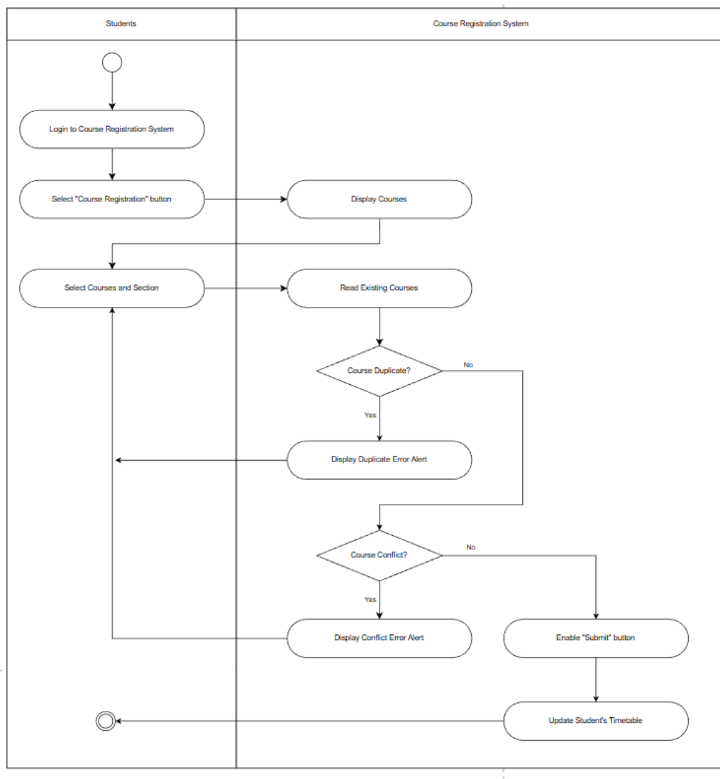
Figure 4.8.3 Activity Diagram for Timetable Conflict Checker Module
